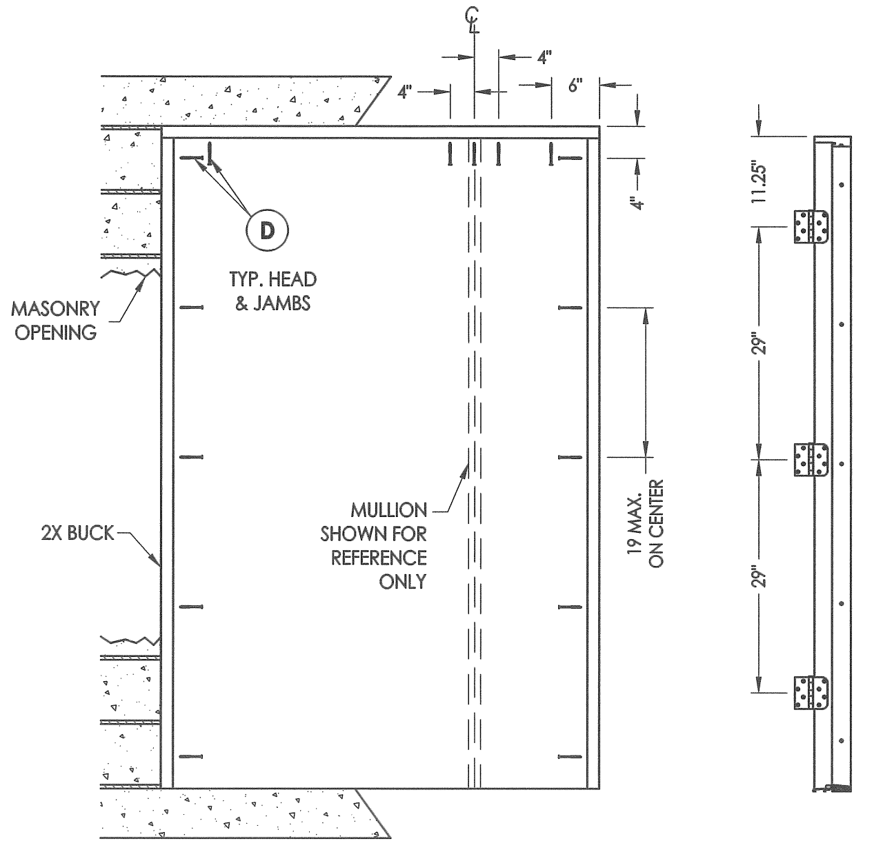
BUCK ANCHORING
